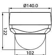
[ LND3110R / LND3210R _ Side / Rear ]
