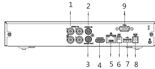
DHI-XVR5108HS-S2
