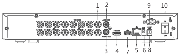
DHI-XVR5116H-S2
