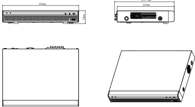
DHI-XVR5116H-S2
