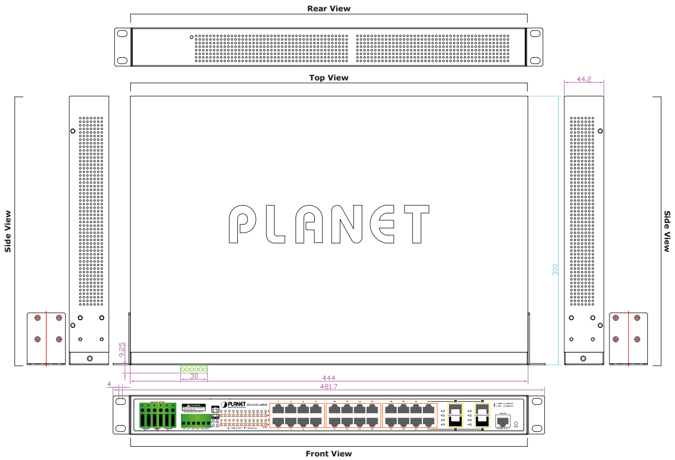
Dimensions (unit = mm)
