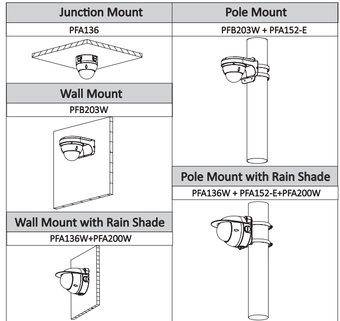
PFA136 Junction Box PFB203W Wall Mount PFA152-E Pole Mount PFA200W Rain shade
