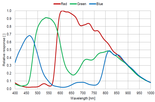
Quantum Efficiency Curve for Color Sensor
