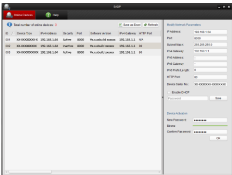
Figure 3-4 SADP Interface
