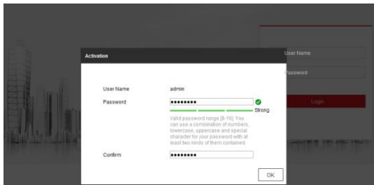
Figure 3-3 Activation Interface(Web)
