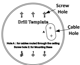
Figure 2. 9 The Drill Template
