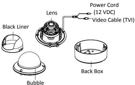
Figure 1. 3 Type III Camera Overview
