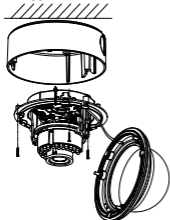
Figure 2. 11 Fix the Camera to the Ceiling
