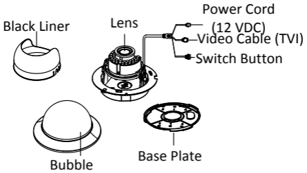
Figure 1. 4 Type IV Camera Overview
