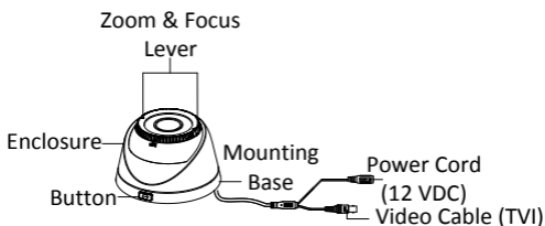
Figure 1. 2 Type II Camera Overview
