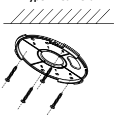
Figure 2. 10 Attach the Back Box/Base Plate
