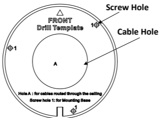
Figure 2. 4 Drill Template
