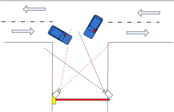
Figure 1-4 Scene 2
