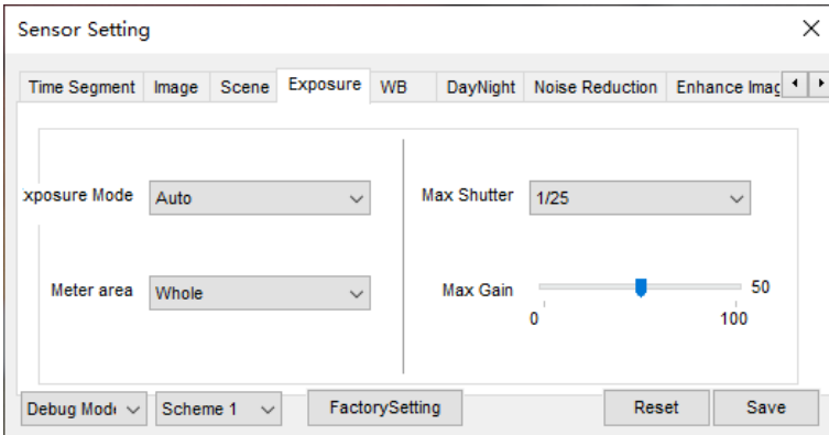
Figure 2-10 Exposure page
