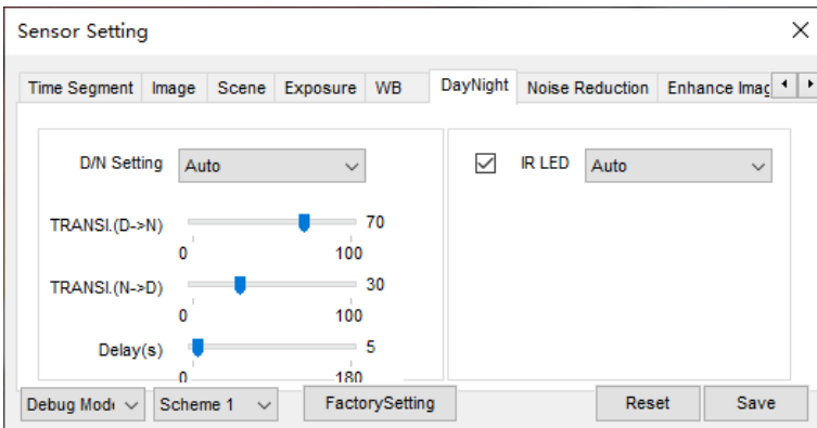
Figure 2-12 DayNight page
