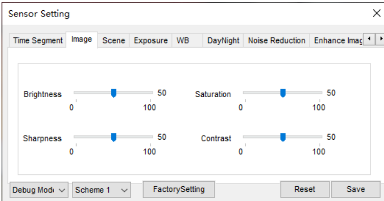
Figure 2-8 Image page
