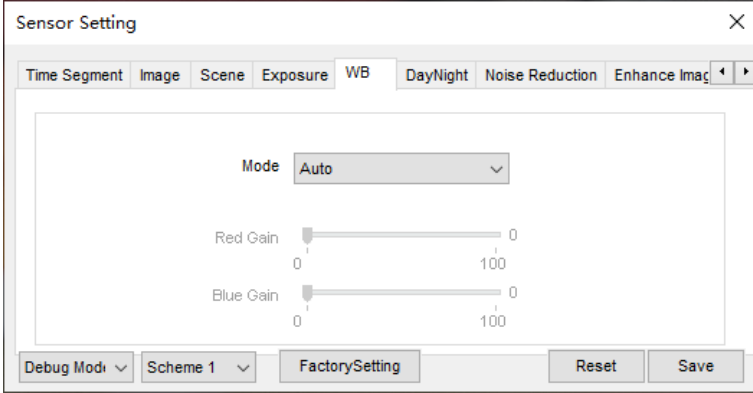
Figure 2-11 WB page
