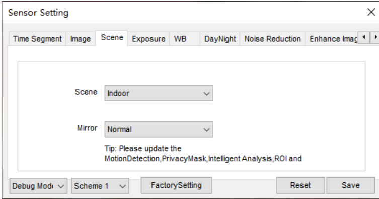
Figure 2-9 Scene page
