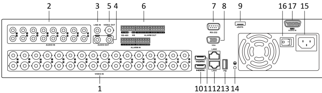
Figure 1-26 Rear Panel of DS-8100HQHI/HUHI-K8 (with 32-ch Video Inputs)
