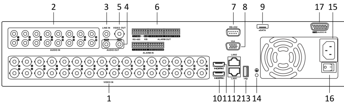
Figure 1-27 Rear Panel of DS-9000HUHI-K8 (with 32-ch Video Inputs)
