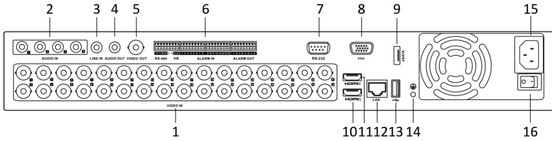
Figure 1-24 Rear Panel of DS-7300HQHI-K4 (with 32-ch Video Inputs)
