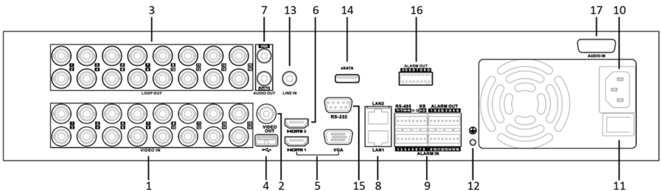
Figure 1-32 Rear Panel of DS-9000HTHI-K8
