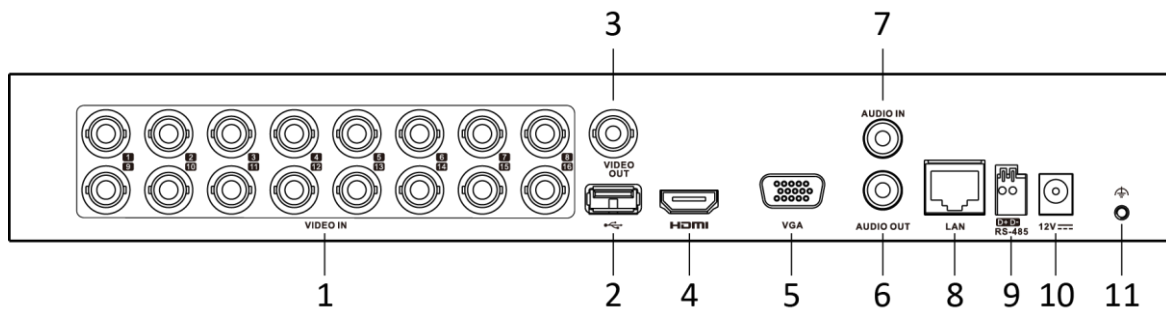
Figure 1-15 Rear Panel of iDS-7200HQHI-K1/S(B), iDS-7200HQHI-M1/S and iDS-7200HQHI-M1/FA (with 16 Video Inputs)
