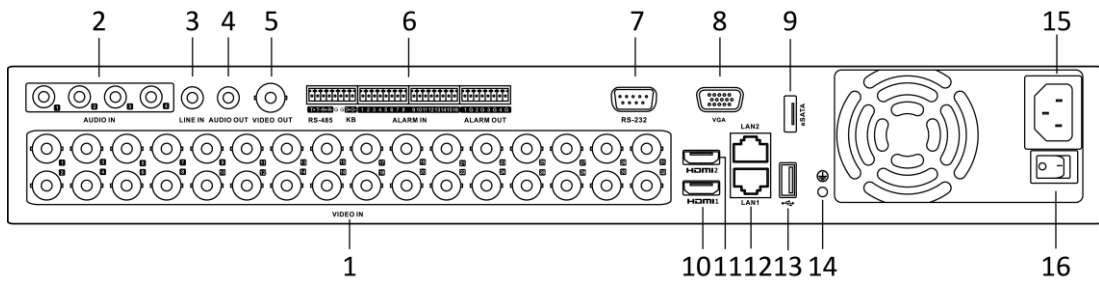
Figure 1-25 Rear Panel of DS-7300HUHI-K4 (with 32-ch Video Inputs)
