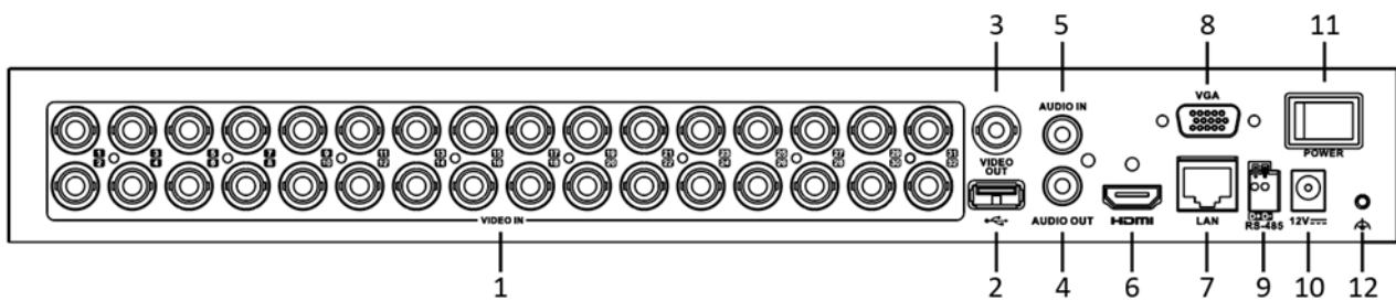
Figure 1-30 Rear Panel of DS-7200HGHI-K2
