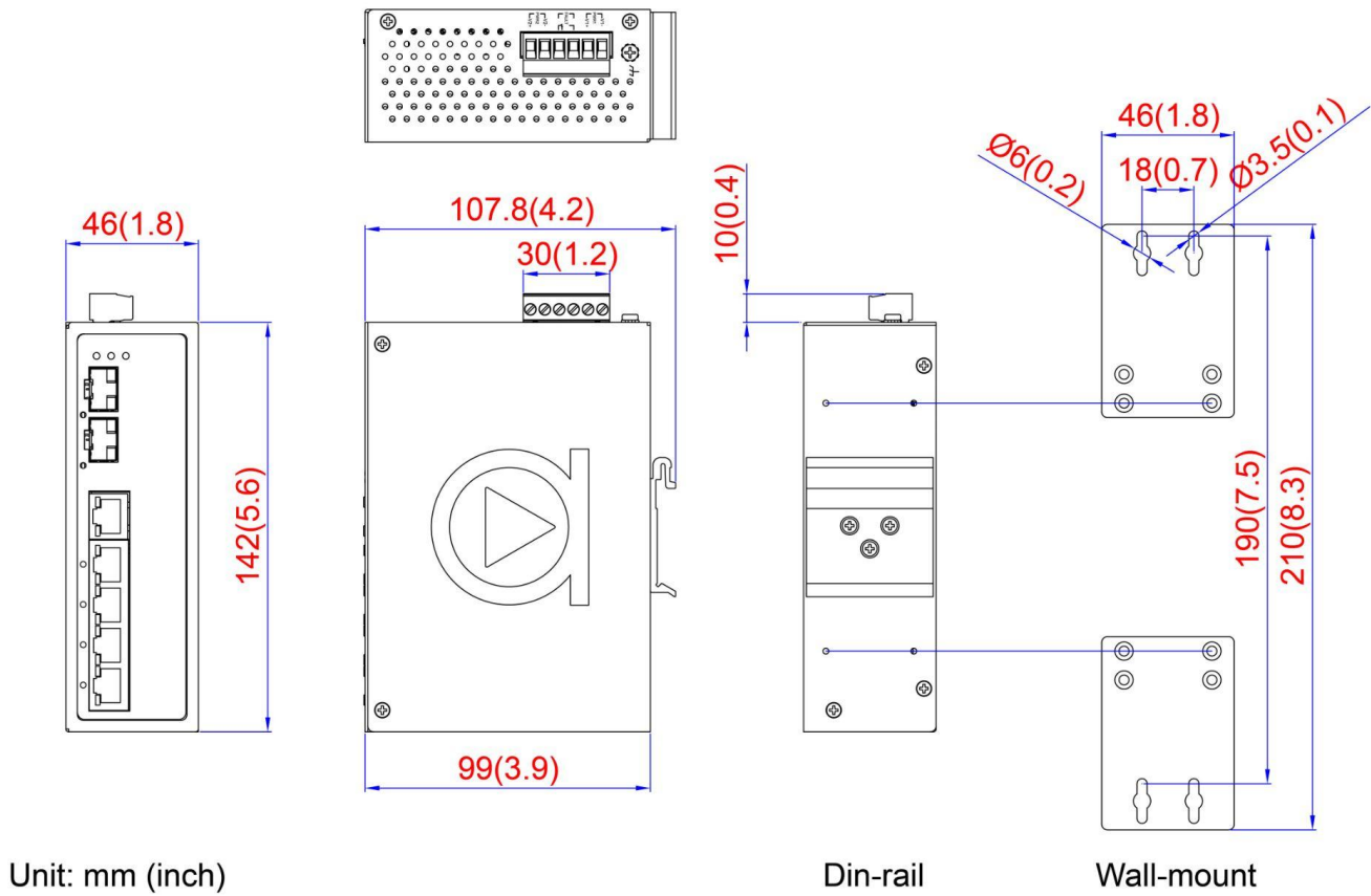
Figure 2.1 - Physical Dimensions
