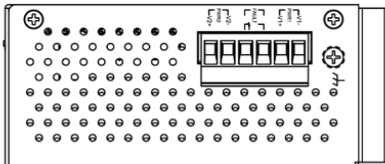
Figure 2.3 - Top View Panel
