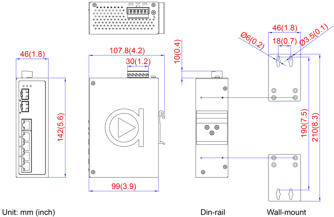
Figure 2.1 - Physical Dimensions
