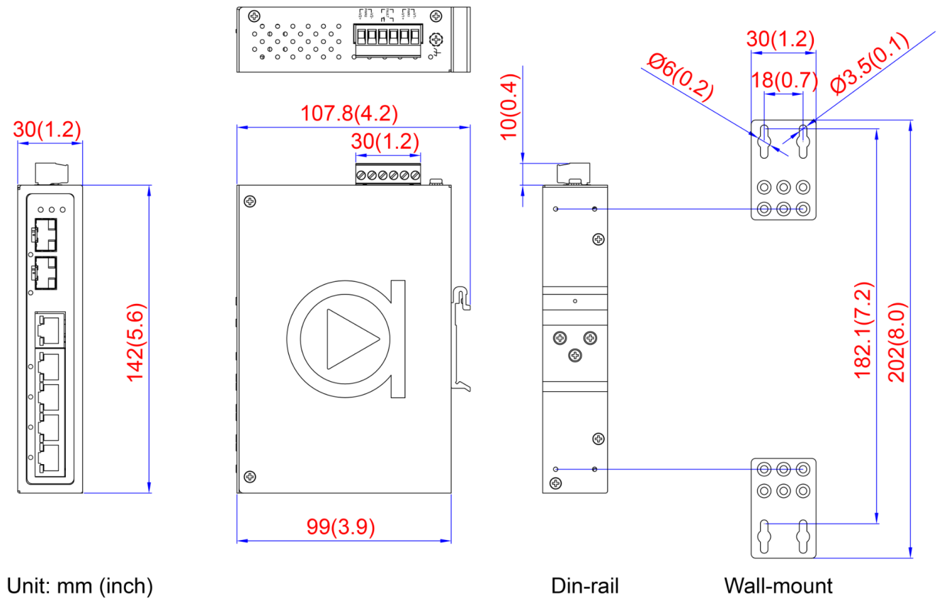
Figure 2.1 - Physical Dimensions
