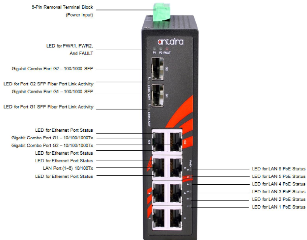
Figure 2.2 - The Front Panel of the LNP-0802C-SFP-24 Series
