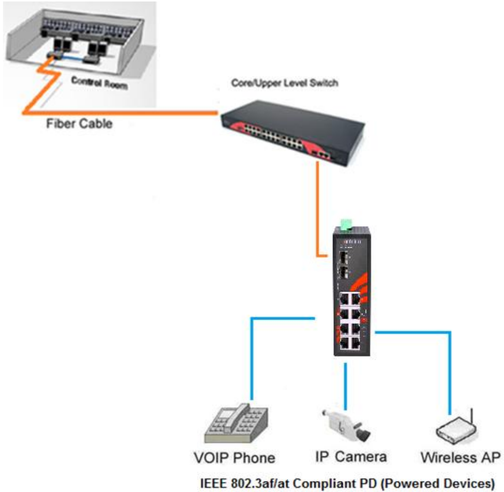
Figure 5.1 Industrial PoE Ethernet Switch Application Reference
