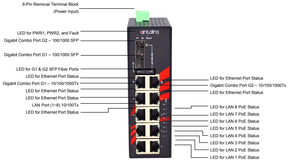
Figure 2.2 - Front Panel of the LNP-1002C-SFP-24 Series
