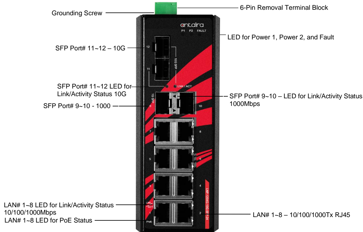
Figure 2.2 - The Front Panel of LNP-1204G-10G-SFP-24
