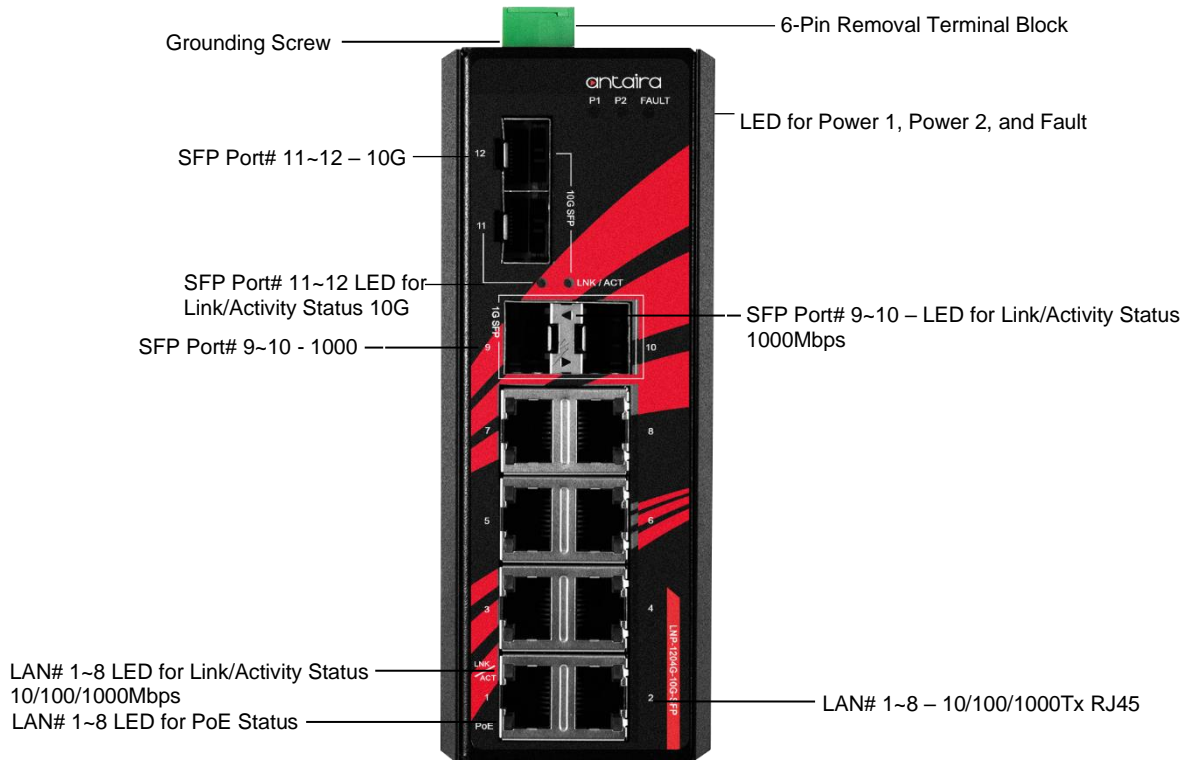
Figure 2.2 - The Front Panel of LNP-1204G-10G-SFP
