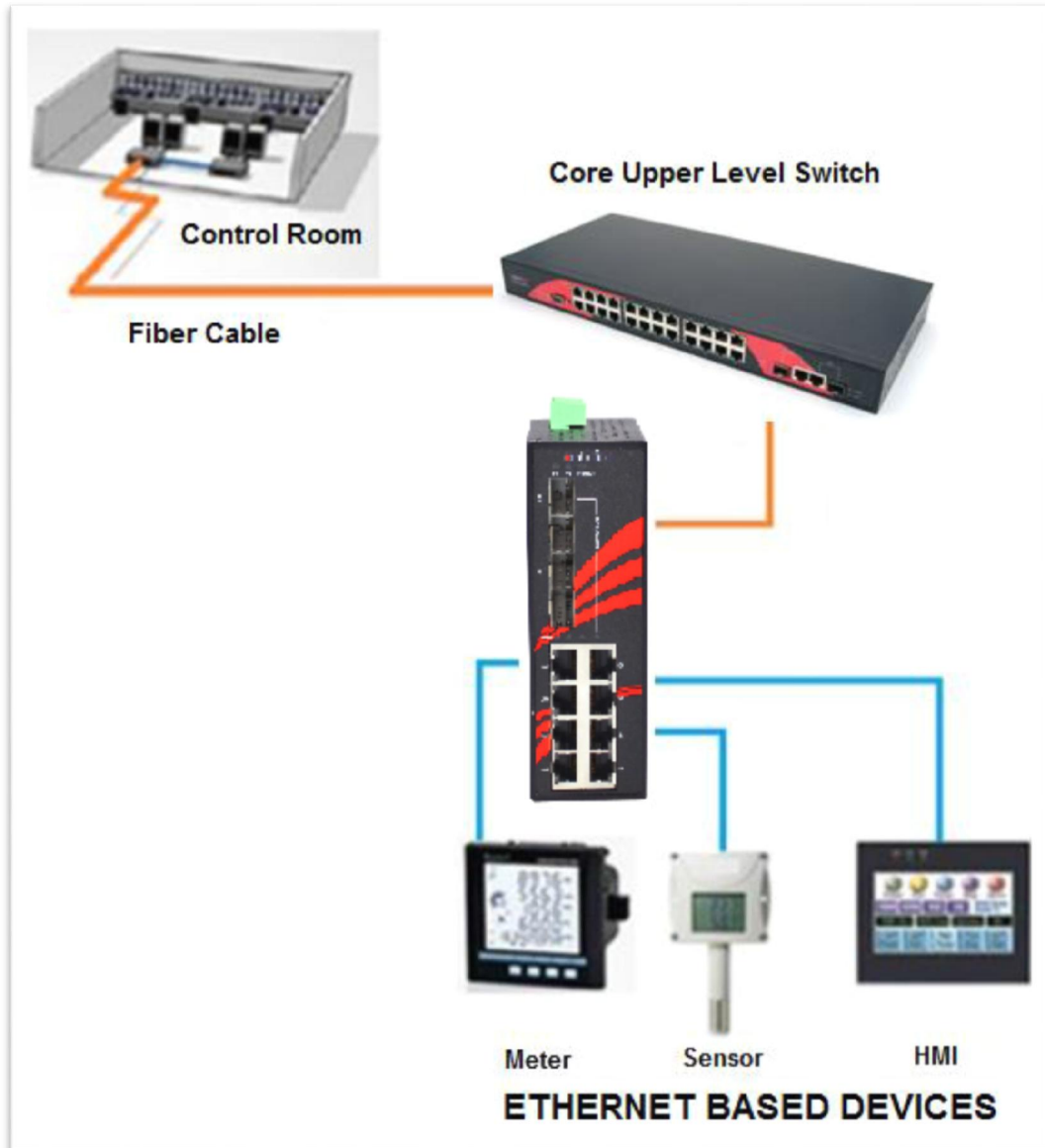
Figure 5.1 Industrial PoE Ethernet Switch Application Reference
