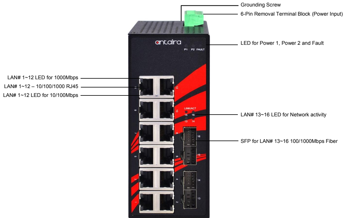
Figure 2.2 - Front Panel of the LNX-1604G-SFP Series
