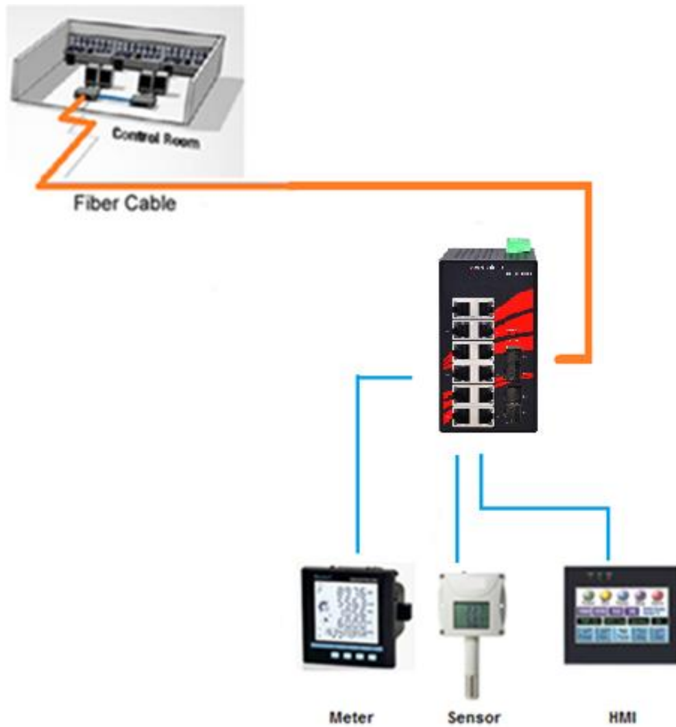
Figure 5.1 Industrial Ethernet Switch Application Reference
